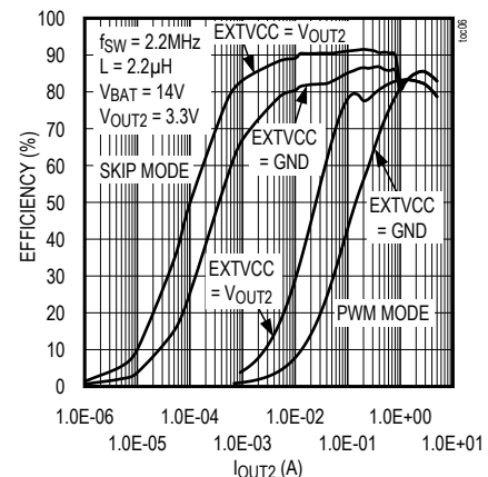
BUCK2 EFFICIENCY
