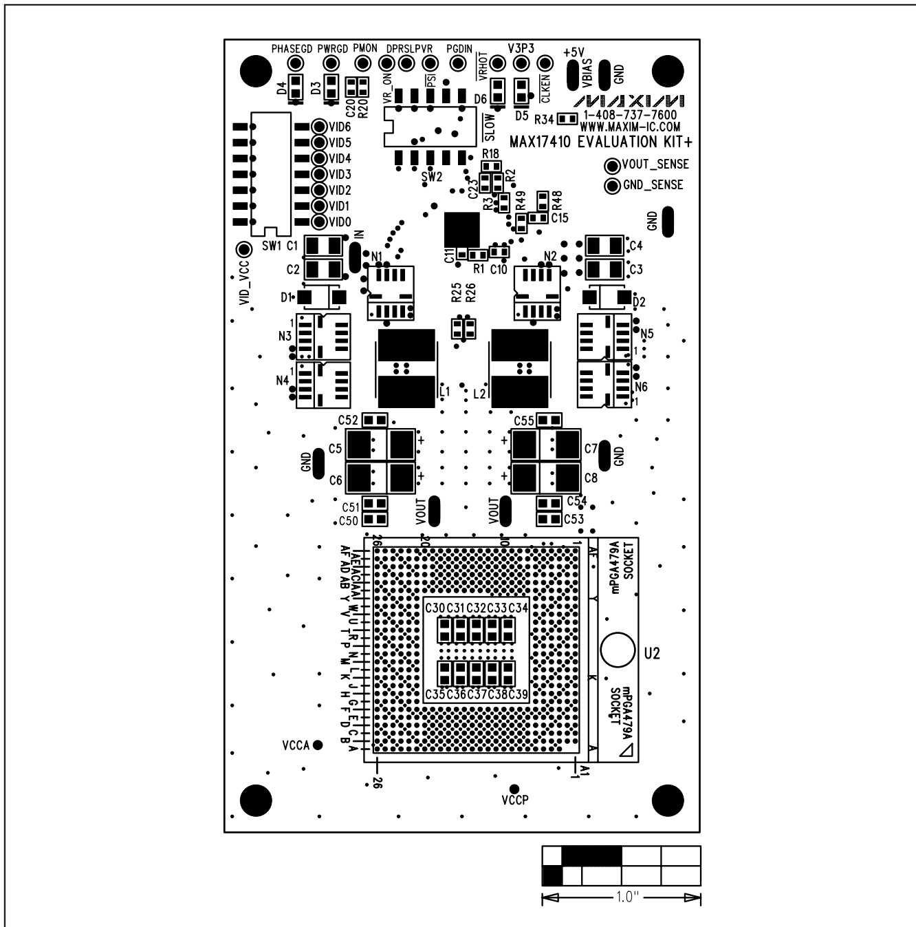
Figure 2. MAX17410 EV Kit Component Placement Guide—Component Side
