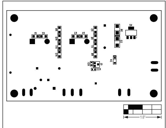
Figure 5. MAX17497A EV Kit Component Placement Guide—Solder Side
