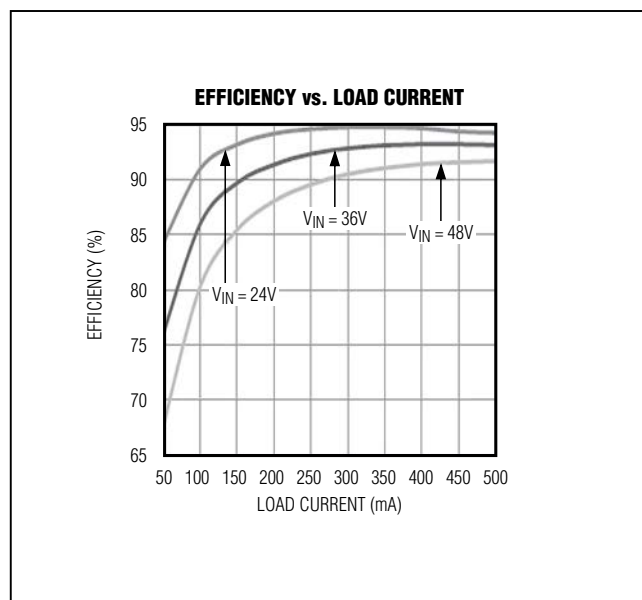
Figure 2. MAX17501G Efficiency
