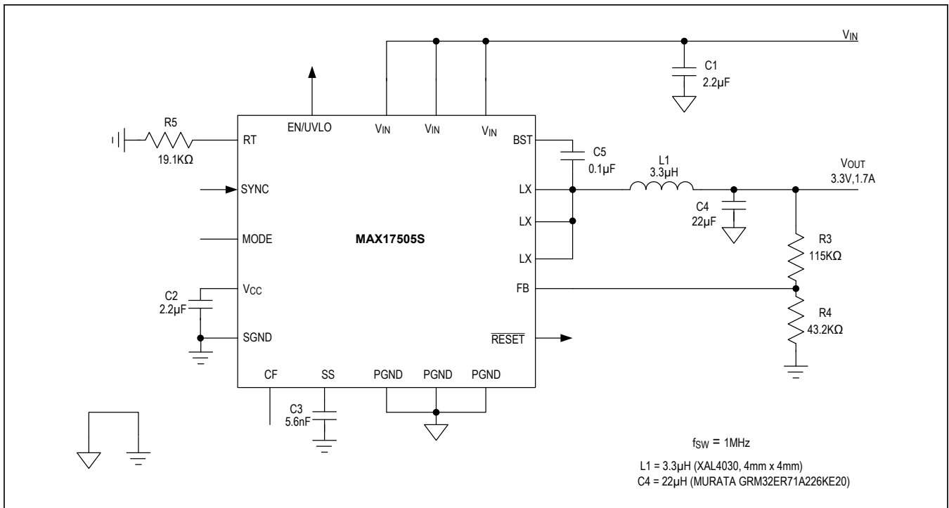
Figure 6. MAX17505S Typical Application Circuit (3.3V Output, 1MHz Switching Frequency)
