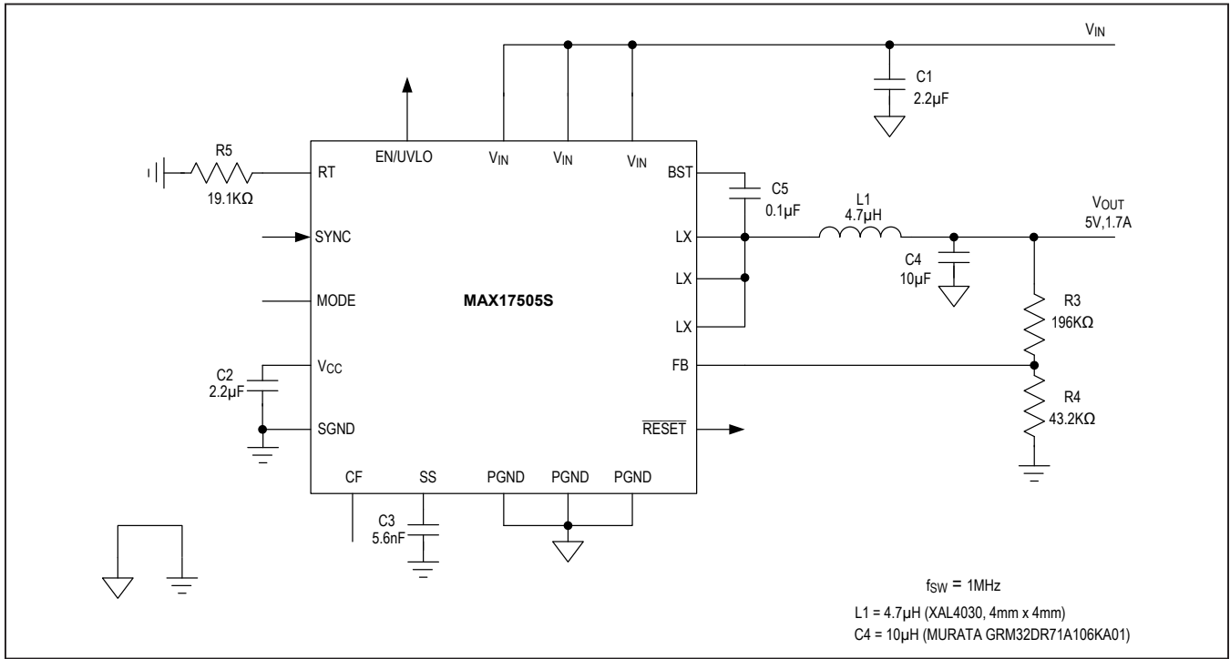
Figure 5. MAX17505S Typical Application Circuit (5V Output, 1MHz Switching Frequency)
