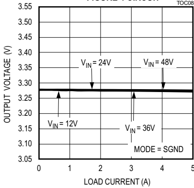
LOAD AND LINE REGULATION 3.3V OUTPUT, PWM MODE, FIGURE 4 CIRCUIT
