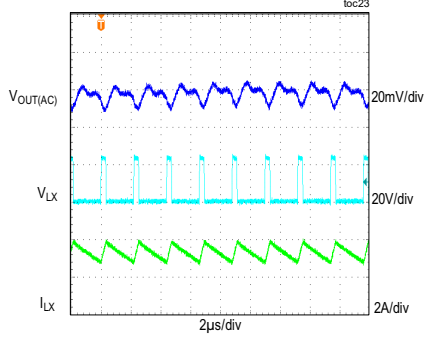
MAX17524, 3.3V OUTPUT STEADY STATE ( f_{sw} = 450kHz , PWM MODE, 3A LOAD)
