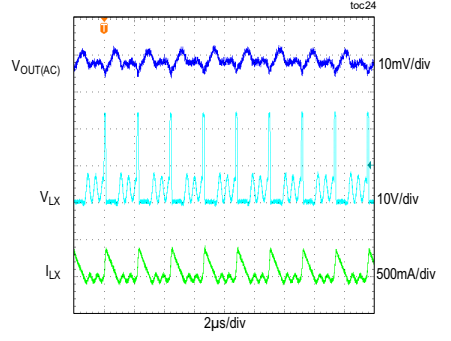
MAX17524, 3.3V OUTPUT STEADY STATE ( f_{sw} = 450kHz , DCM MODE, 75mA LOAD)
