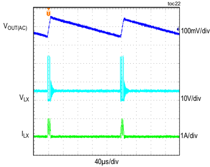
MAX17524, 5V OUTPUT STEADY STATE ( f_{sw} = 450kHz , PFM MODE, 25mA LOAD)
