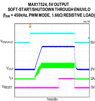
CONDITION: RESET IS PULLED UP TO V_{CC}
