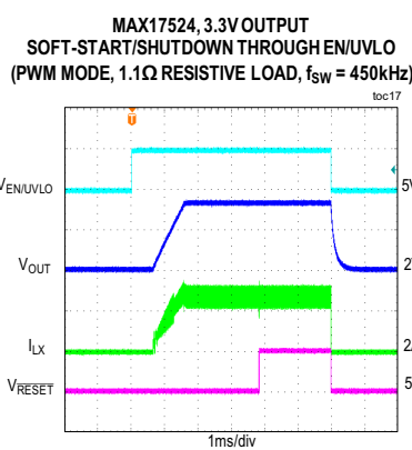
CONDITION: RESET IS PULLED UP TO V_{CC}
