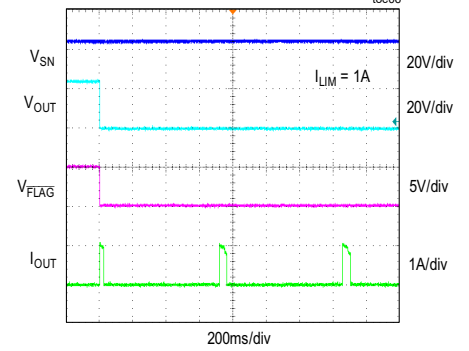
AUTORETRY CURRENT-LIMIT RESPONSE toc06
