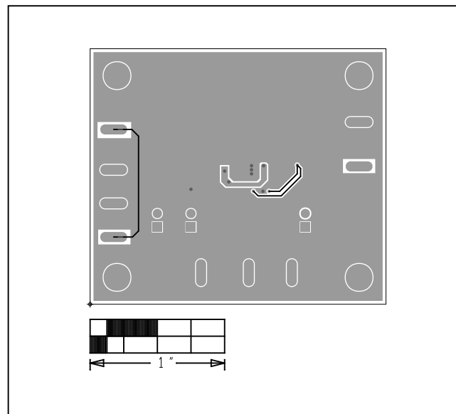
Figure 3. MAX17550 5V EV Kit (TDFN) PCB Layout—Solder Side
