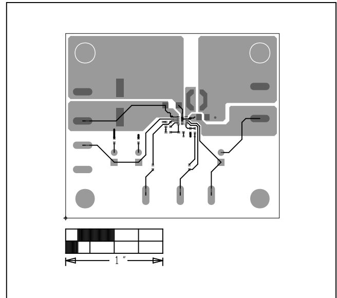
Figure 2. MAX17550 5V EV Kit (TDFN) PCB Layout—Component Side
