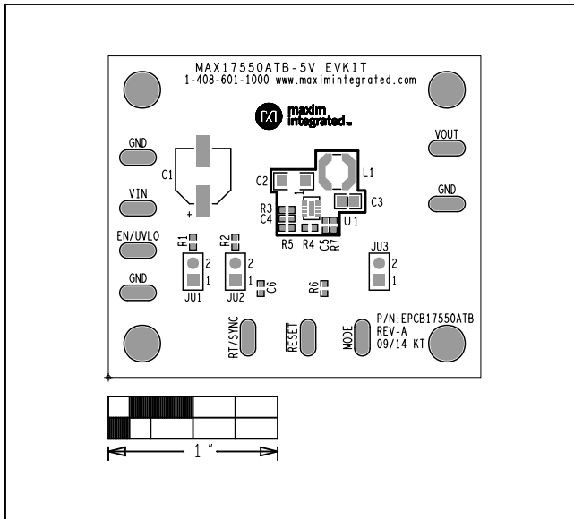
Figure 1. MAX17550 5V EV Kit (TDFN) Component Placement Guide—Component Side
