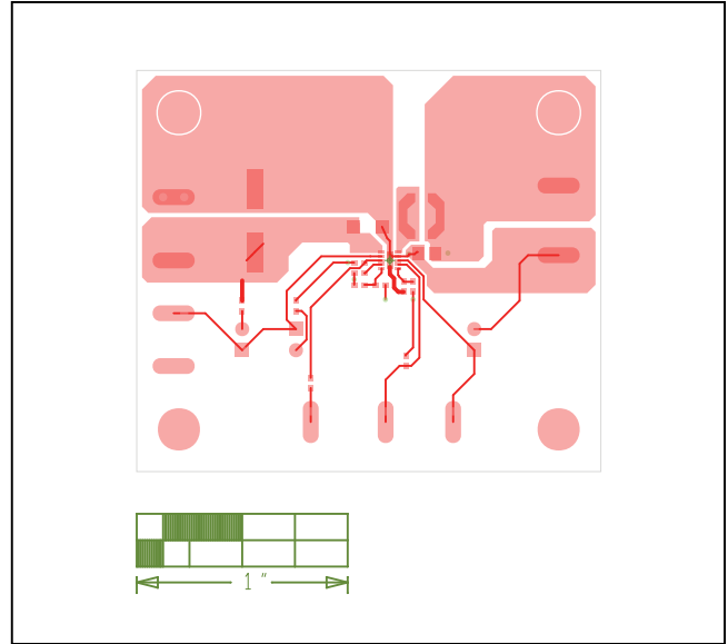
Figure 2. MAX17551 5V EV Kit (TDFN) PCB Layout—Component Side
