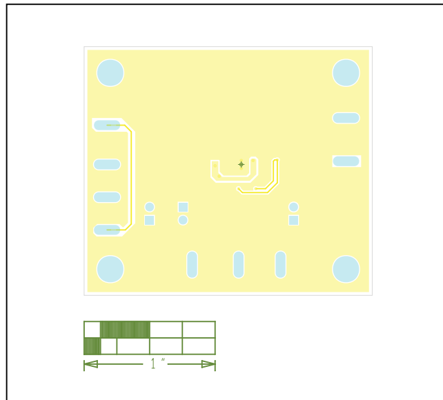
Figure 3. MAX17551 5V EV Kit (TDFN) PCB Layout—Solder Side
