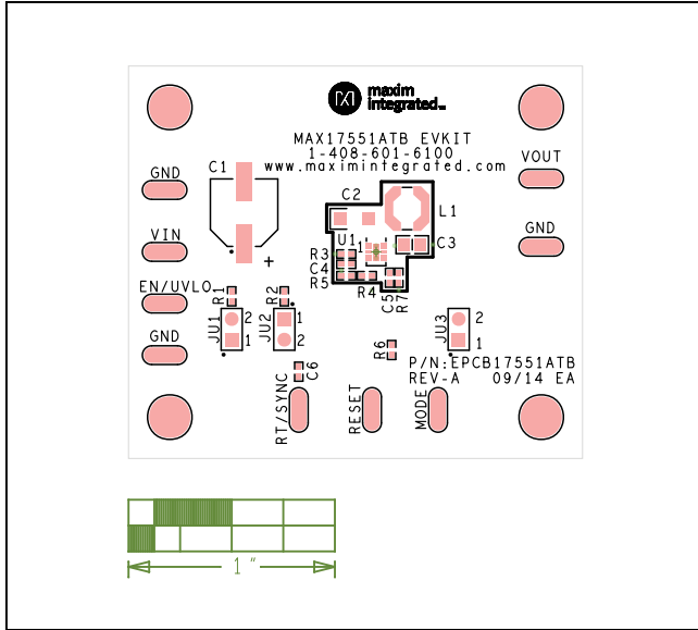
Figure 1. MAX17551 5V EV Kit (TDFN) Component Placement Guide—Component Side
