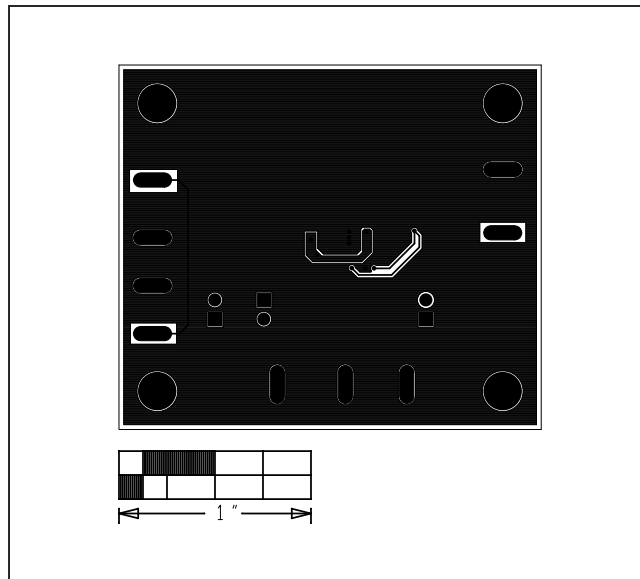
MAX17552 5V EV Kit (TDFN)—Bottom Layer
