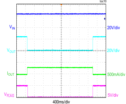
OVERCURRENT FAULT RESPONSE AND RECOVERY
