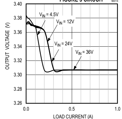
MAX17630A LOAD AND LINE REGULATION FIGURE 3 CIRCUIT
