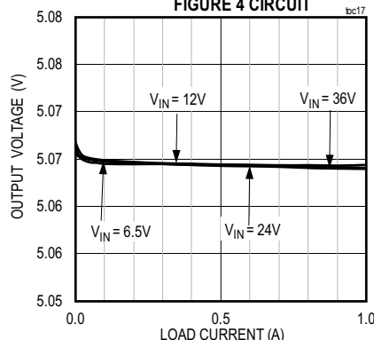
MAX17630B LOAD AND LINE REGULATION FIGURE 4 CIRCUIT
