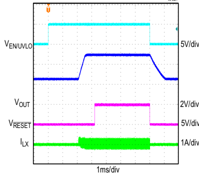
MAX17630C SOFT-START WITH PREBIAS VOLTAGE OF 2.5V FIGURE 7 CIRCUIT
