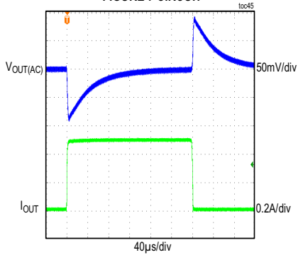
MAX17630C LOAD TRANSIENT BETWEEN 0A AND 0.5A FIGURE 7 CIRCUIT
