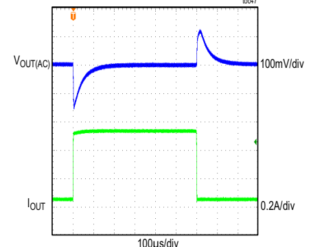
MAX17630C LOAD TRANSIENT BETWEEN 20mA AND 0.5A FIGURE 7 CIRCUIT
