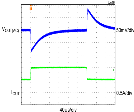
MAX17630C LOAD TRANSIENT BETWEEN 0.5A AND 1A FIGURE 7 CIRCUIT
