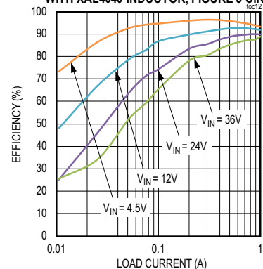
MAX17630A EFFICIENCY vs. LOAD CURRENT WITH XAL4040 INDUCTOR, FIGURE 3 CIRCUIT
