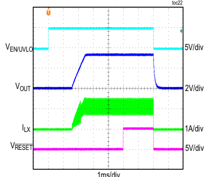
MAX17630A SOFT-START/SHUTDOWN FROM EN/UVLO FIGURE 3 CIRCUIT toc22
