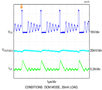
STEADY-STATE PERFORMANCE
