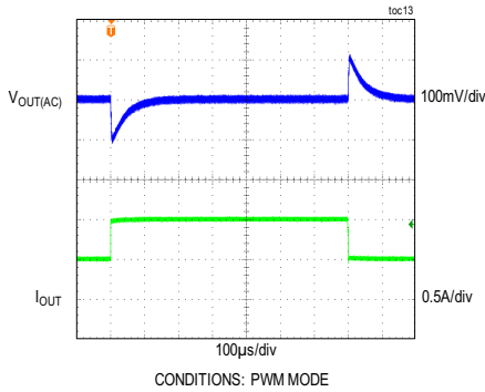
LOAD TRANSIENT RESPONSE BETWEEN 0.5A AND 1A
