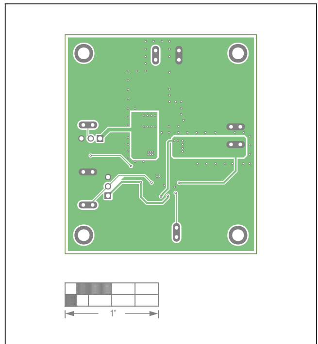
MAX17630BEVKIT# EV Kit—Layer 3
