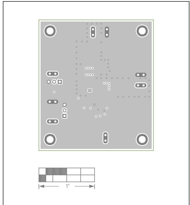
MAX17630BEVKIT# EV Kit—Layer 2
