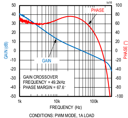
BODE PLOT
