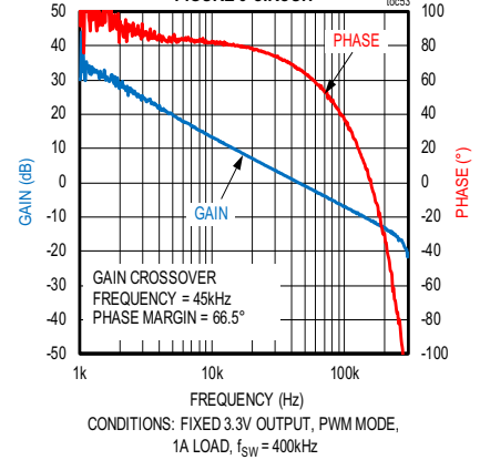
MAX17630A CLOSED-LOOP BODE PLOT FIGURE 3 CIRCUIT
