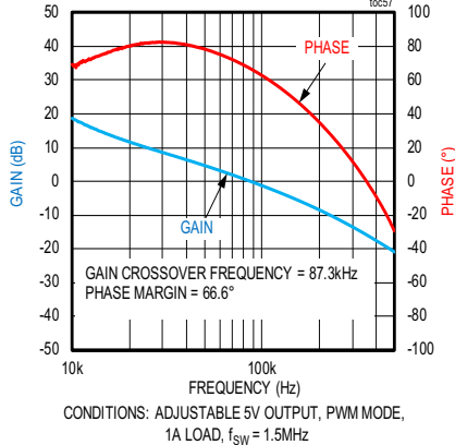
MAX17630C CLOSED-LOOP BODE PLOT FIGURE 7 CIRCUIT
