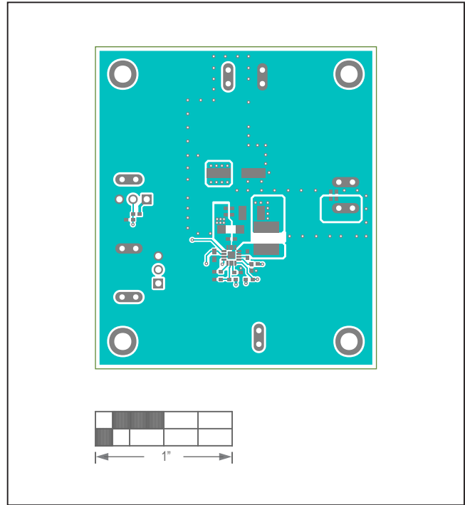
MAX17631C5EVKIT# EV Kit—Top Layer
