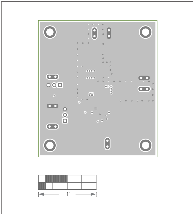
MAX17631C5EVKIT# EV Kit—Layer 2
