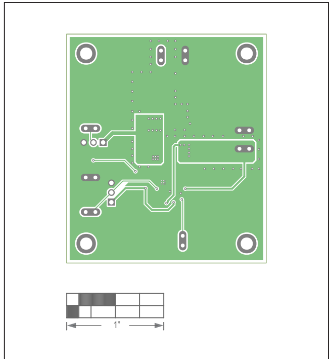
MAX17631C5EVKIT# EV Kit—Layer 3
