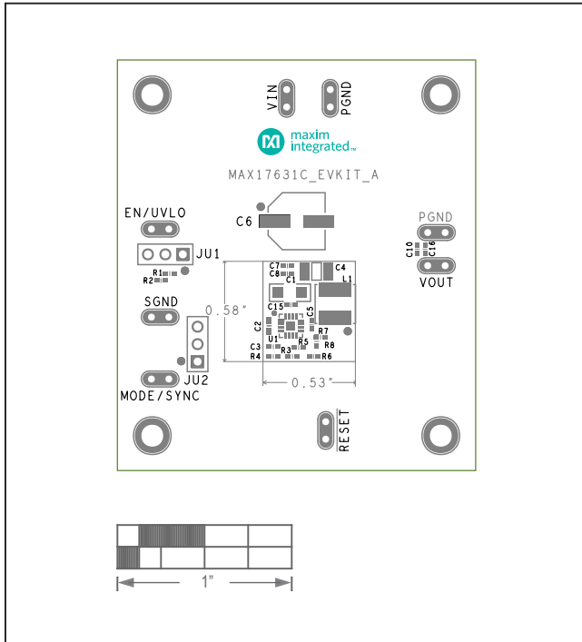
MAX17631C5EVKIT# EV Kit—Top Silkscreen
