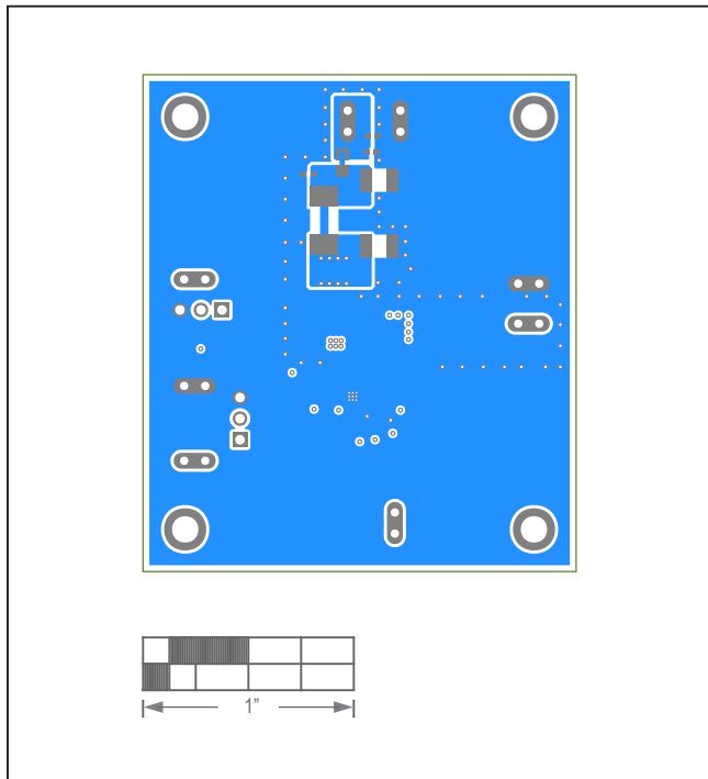
MAX17631C5EVKIT# EV Kit—Bottom Layer
