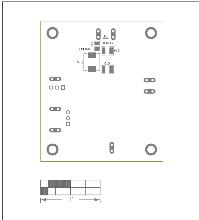
MAX17631C5EVKIT# EV Kit—Bottom Silkscreen
