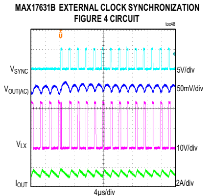
CONDITIONS: FIXED 5V OUTPUT, PWM MODE, 1.5A LOAD CURRENT f_{SW} = 400kHz , EXTERNAL CLOCK FREQUENCY = 440kHz
