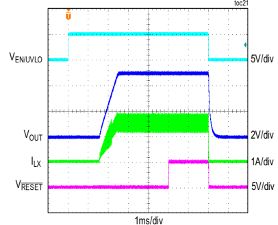
MAX17631B SOFT-START/SHUTDOWN FROM EN/UVLO FIGURE 4 CIRCUIT
