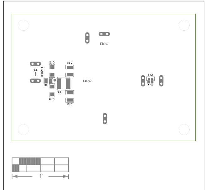
MAX17634A EV Kit—Bottom Silkreen
