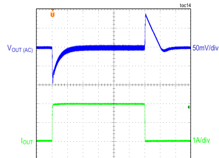
CONDITIONS: DCM MODE
