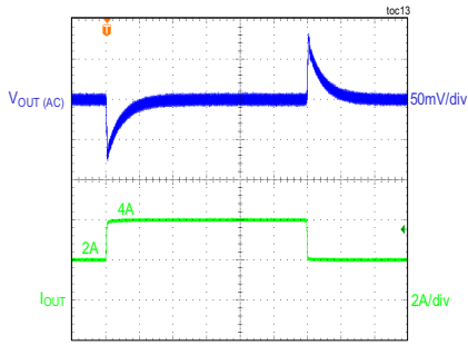
CONDITIONS: PWM/PPM/DCM MODE
