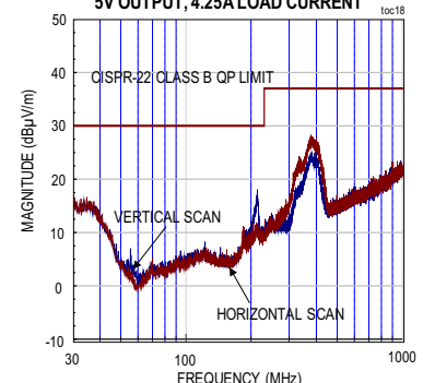
CONDITIONS: L2 = SHORT, C12 = C13 = C14 = C19 = OPEN
