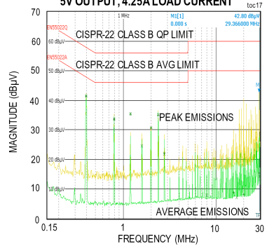
CONDITIONS: L2 = 22µH, C12 = C13 = 2.2µF/50V/X7R/1206, C14 = C19 = 4.7µF/50V/X7R/1210
