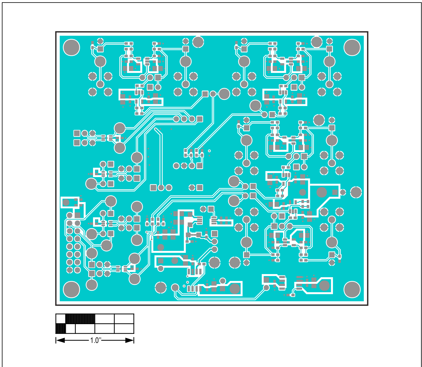
MAX19777 EV Kit—PCB Top View
