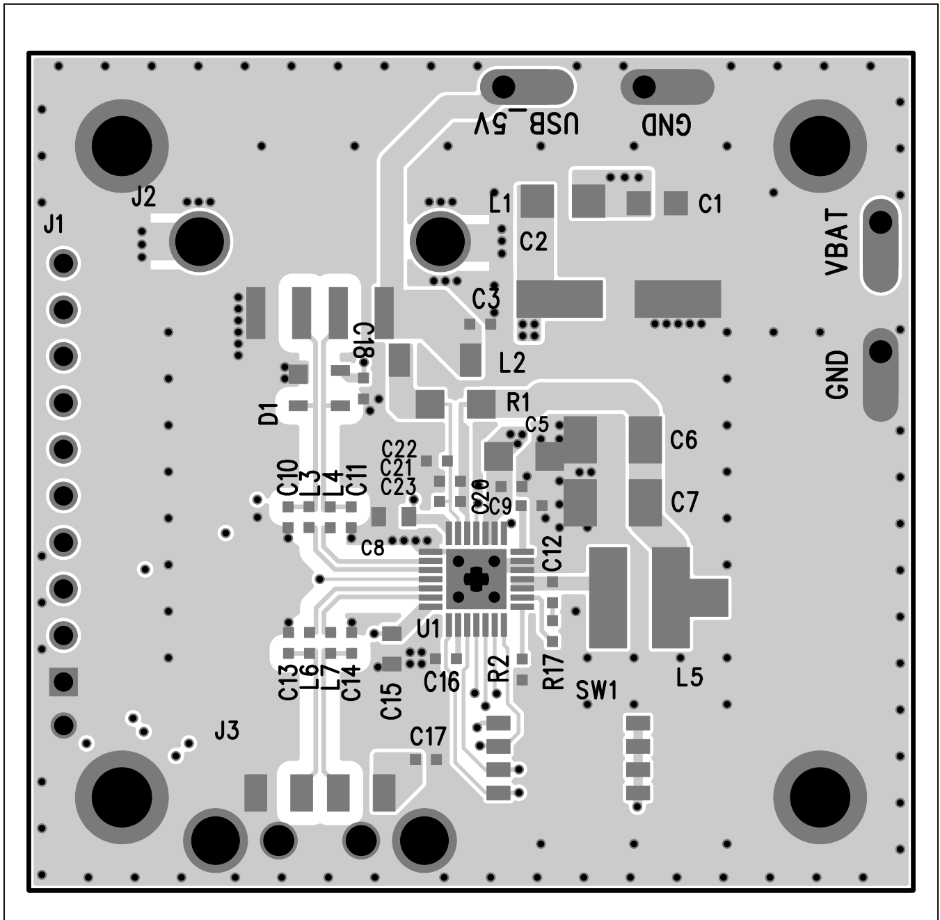
MAX20038 EV Kit PCB Layout—Top Layer
