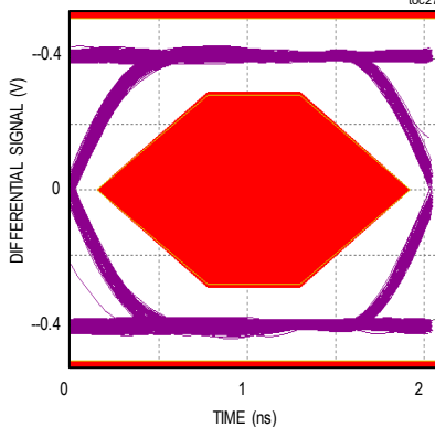
REFERENCE HIGH-SPEED EYE DIAGRAM (NO MAX20046) toc27
