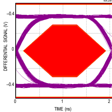
USB 2.0 HIGH-SPEED EYE DIAGRAM (NO TUNING COMPONENTS) toc28
