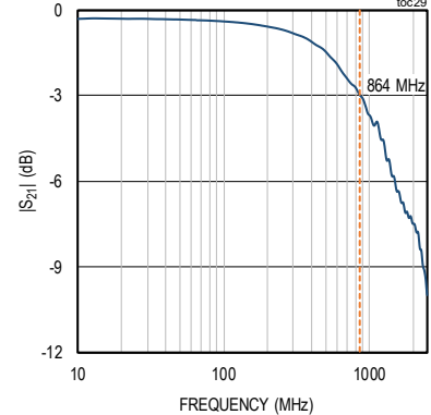
SINGLE-ENDED BANDWIDTH toc29
