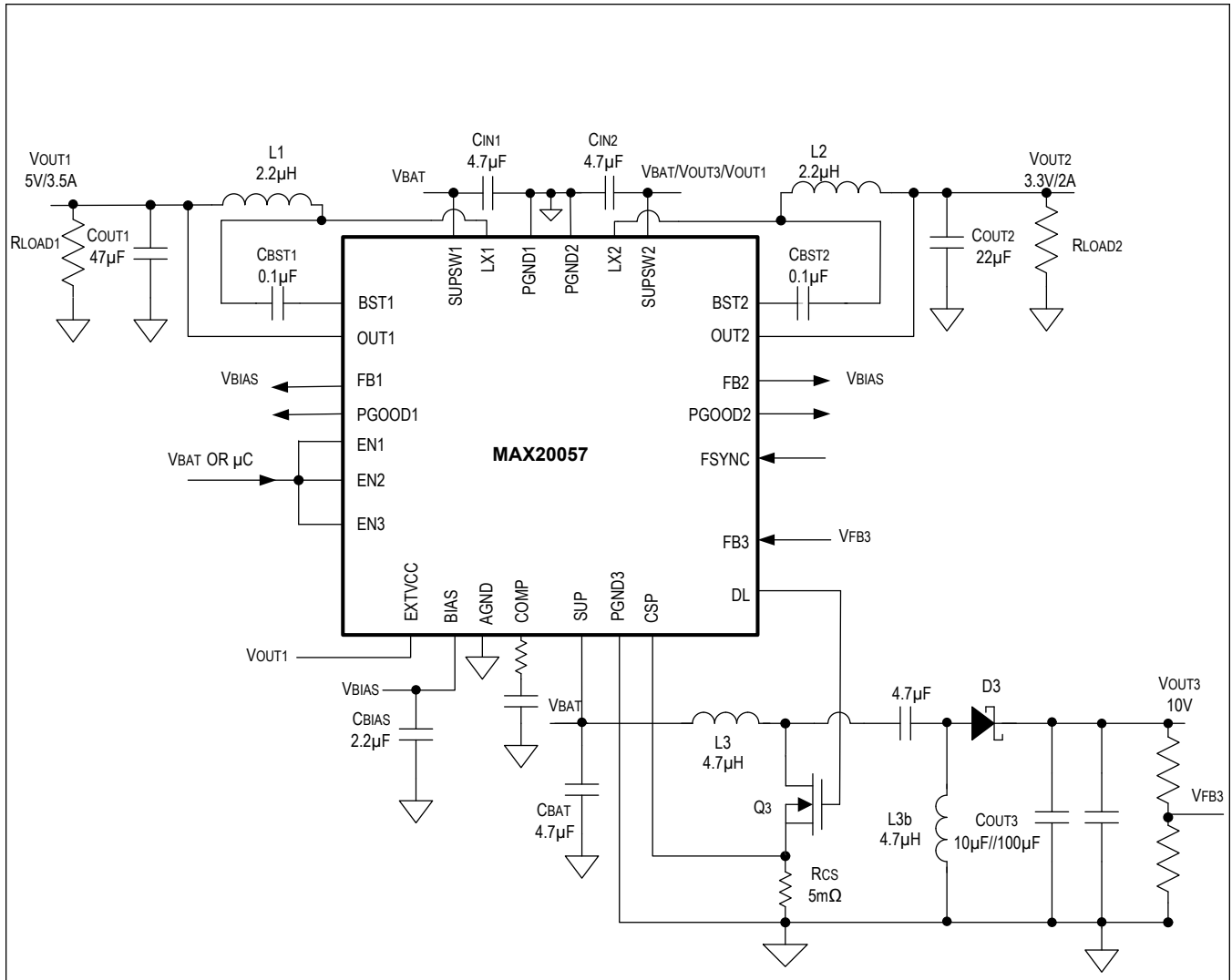
Figure 2. MAX20057 SEPIC Application Circuit
