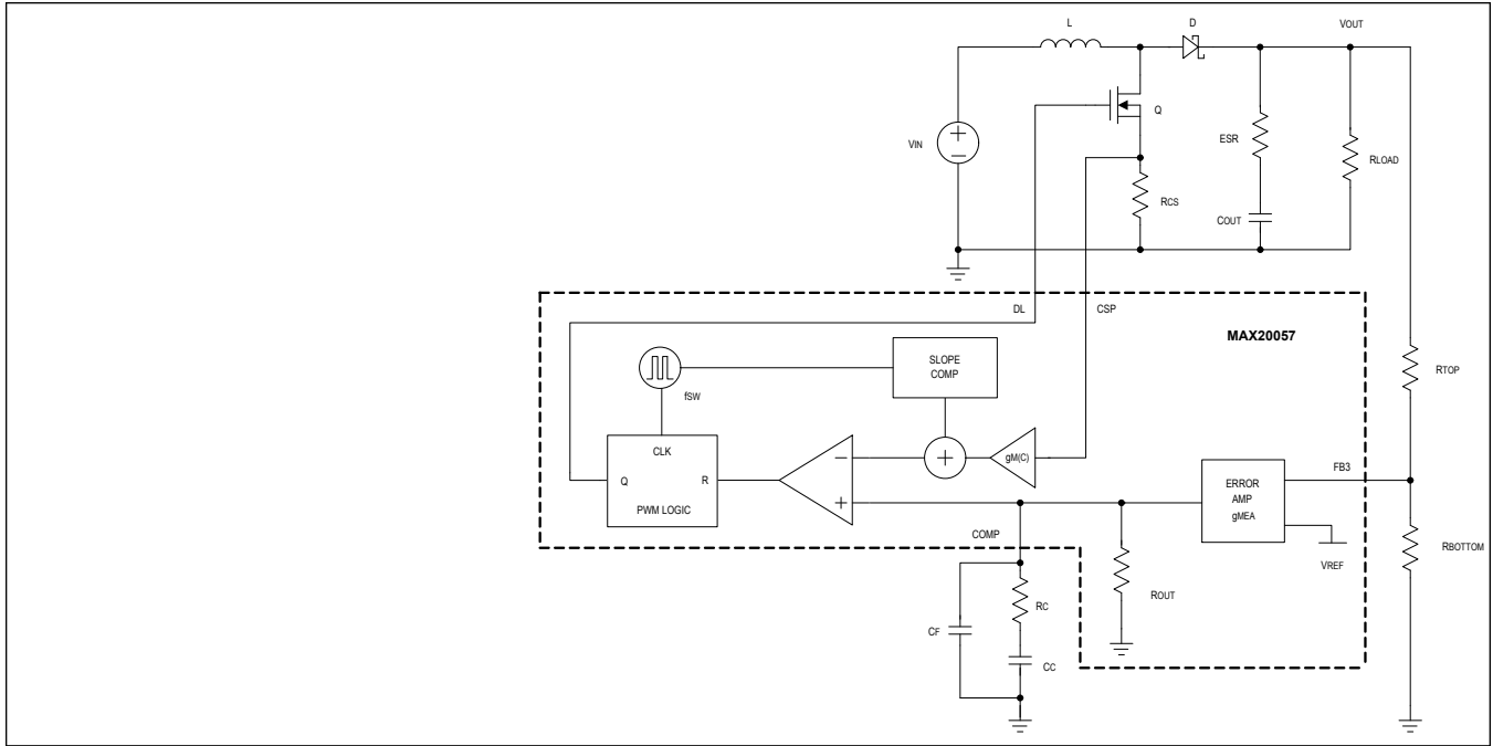
Figure 1. Boost Control Loop
