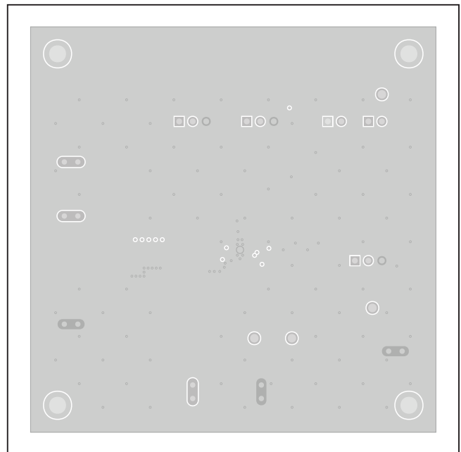
MAX20077 EV Kit PCB Layout—Internal Layer 3
