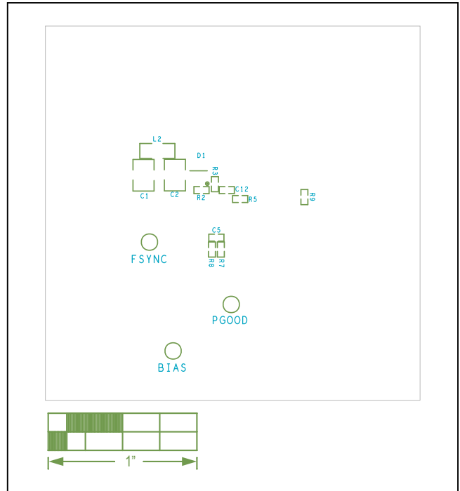
MAX20098 EV Kit Component Placement Guide—Silkscreen (Bottom)
