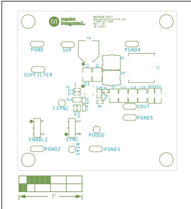
MAX20098 EV Kit Component Placement Guide—Silkscreen (Top)
