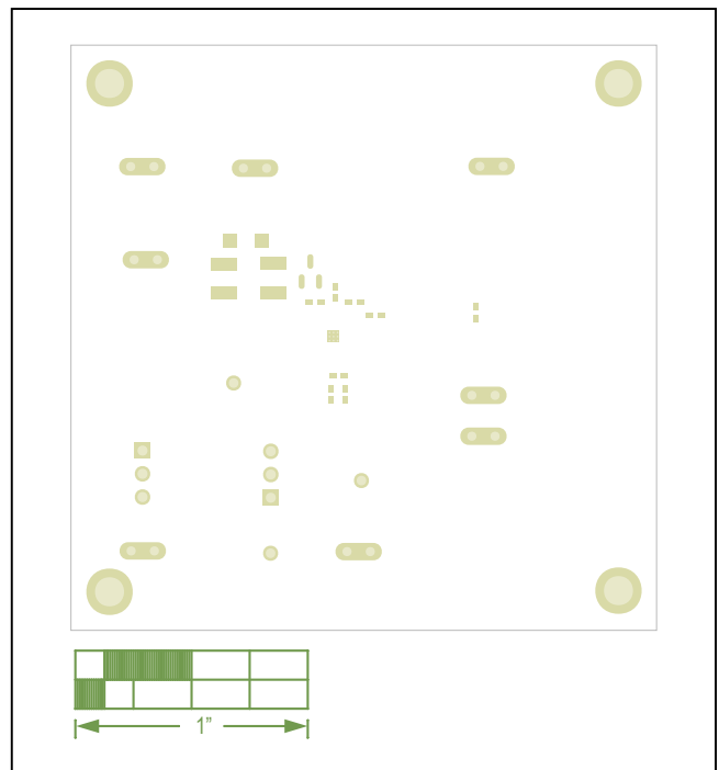
MAX20098 EV Kit PCB Layout—Soldermask (Bottom)
