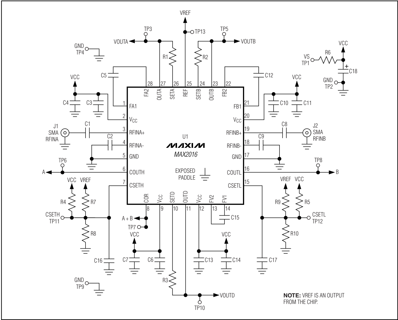
Figure 4. MAX2016 EV Kit Schematic
