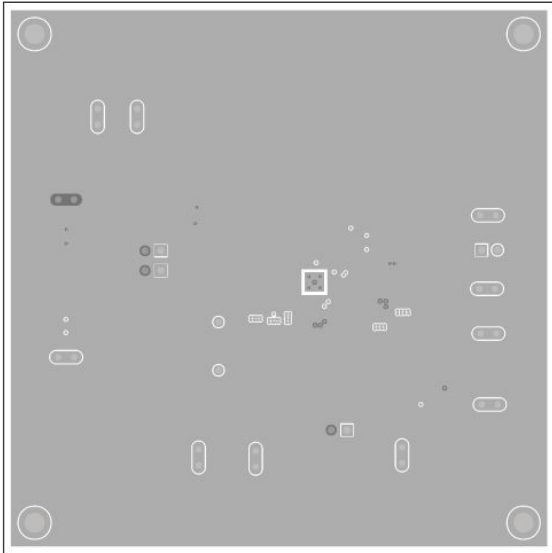
MAX20414 EV Kit Schematic PCB Layout—Internal Layer 3
