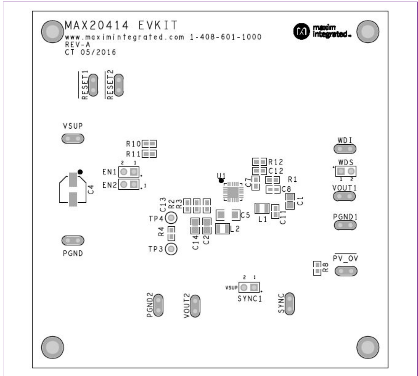
MAX20414 EV Kit Schematic Component Placement Guide—Top Silkscreen
