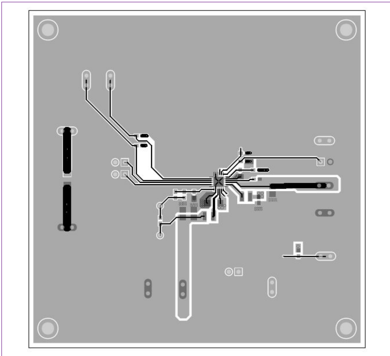
MAX20414 EV Kit Schematic PCB Layout—Top Layer
