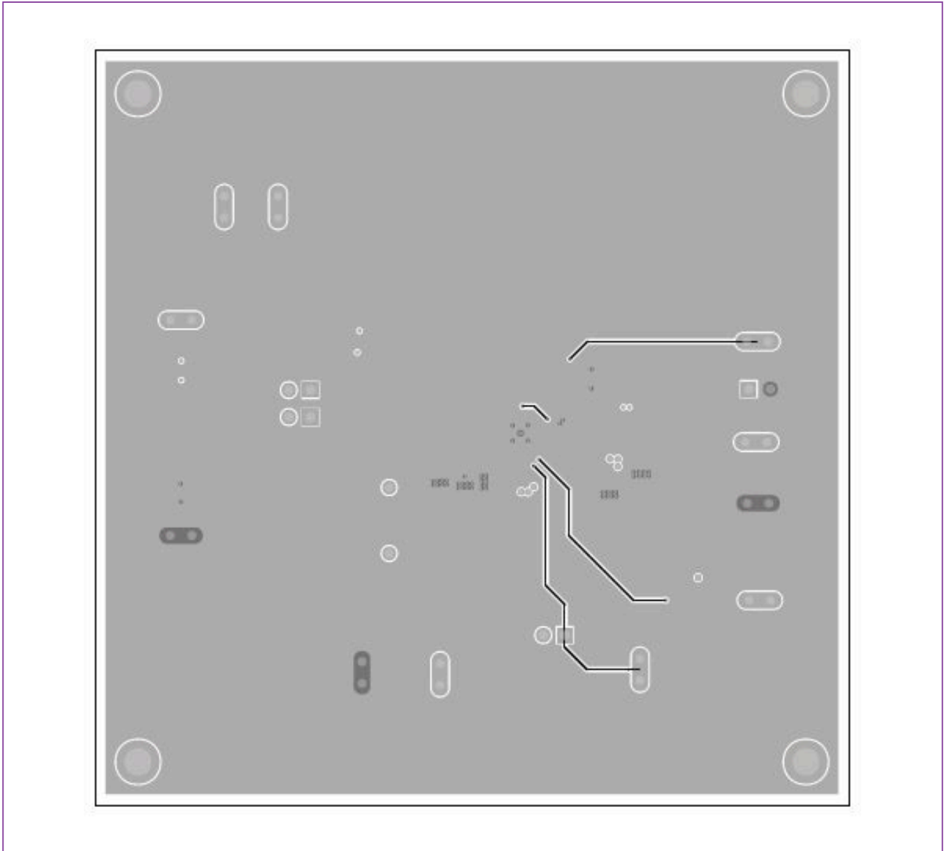
MAX20414 EV Kit Schematic PCB Layout—Bottom Layer
