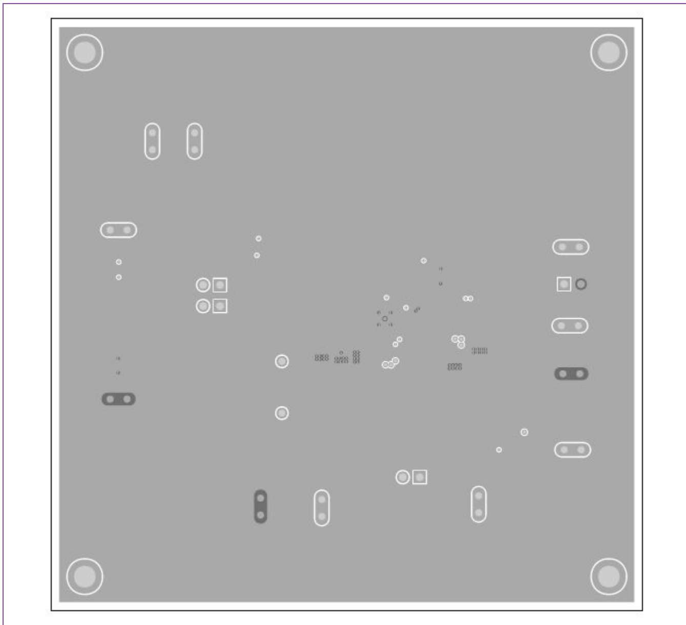
MAX20414 EV Kit Schematic PCB Layout—Internal Layer 2
