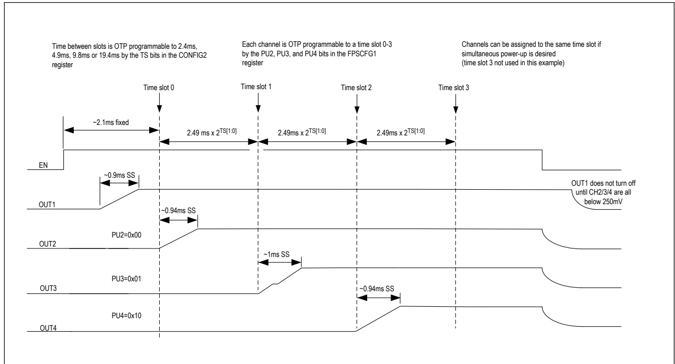
Figure 2. Flexible Power Sequencer Timing
