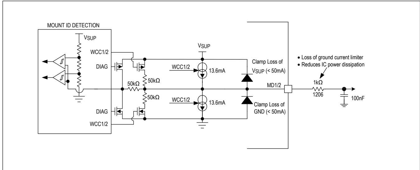
Figure 4. Mount ID Detection (One Channel Shown)
