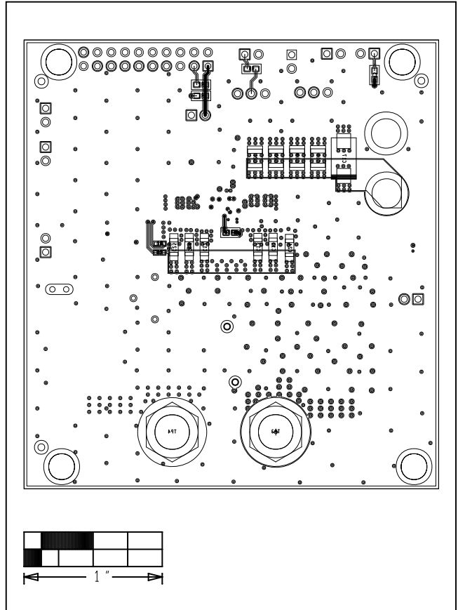
Figure 11. MAX20499C EV Kit PCB Layout—Bottom Layer
