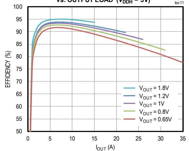
SYSTEM EFFICIENCY vs. OUTPUT LOAD ( V_{DDH} = 5V )
