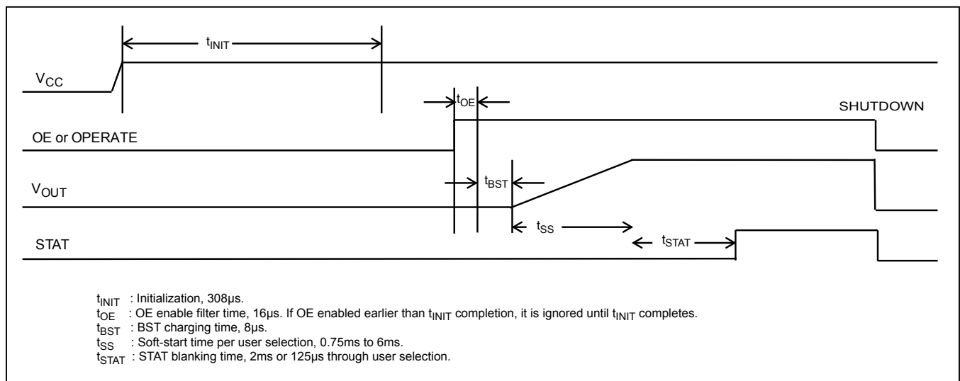
Figure 1. Startup Timing
