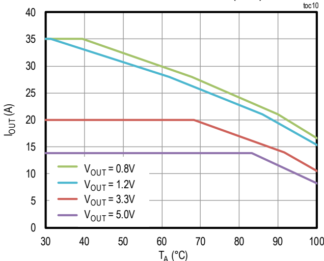
SAFE OPERATING AREA (SOA)
