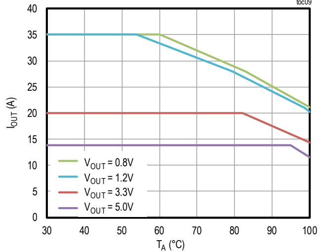
SAFE OPERATING AREA (SOA)
