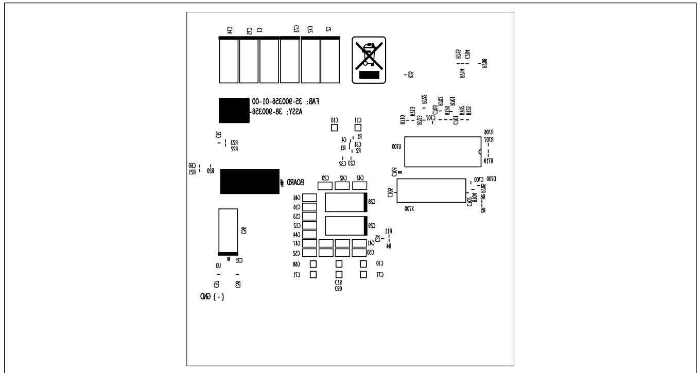
Bottom Silkscreen
