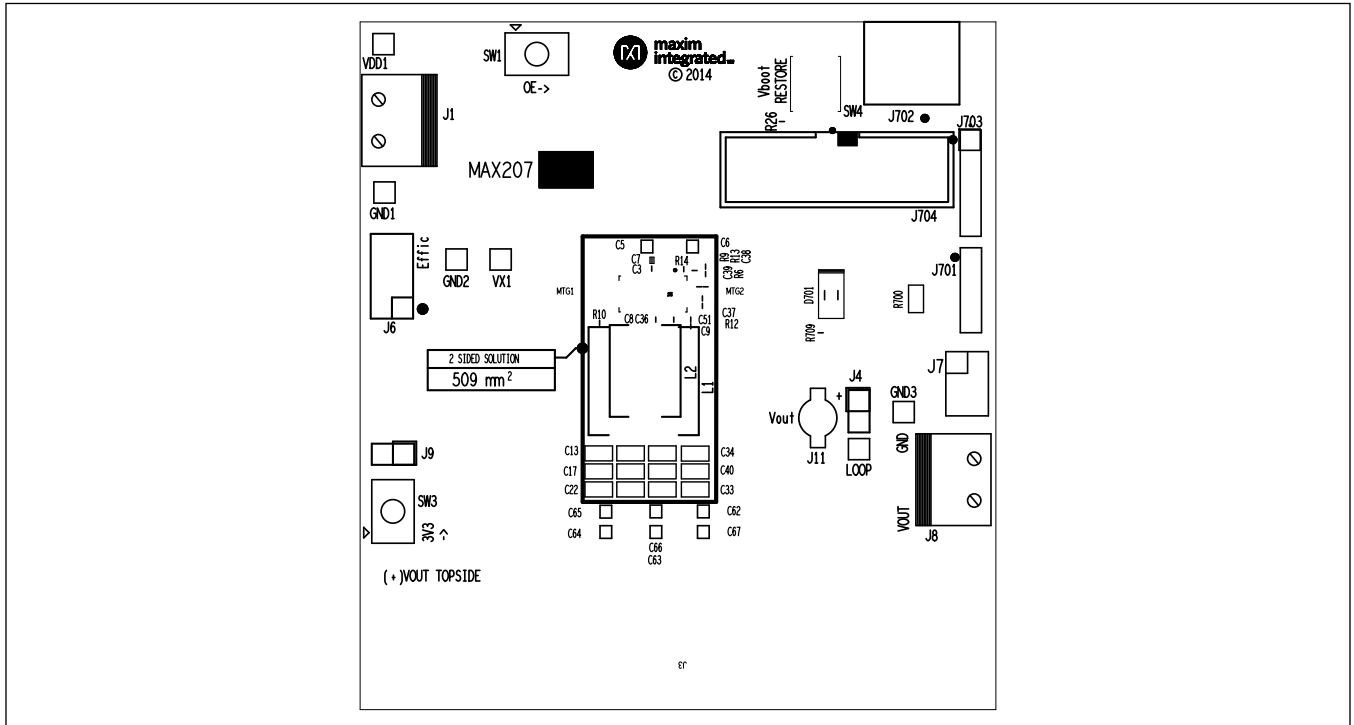
Top Silkscreen
