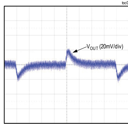
TIME: 50µs/div CONDITIONS: I_{OUT} = 20A to 30A STEP at 1A/\mu s
