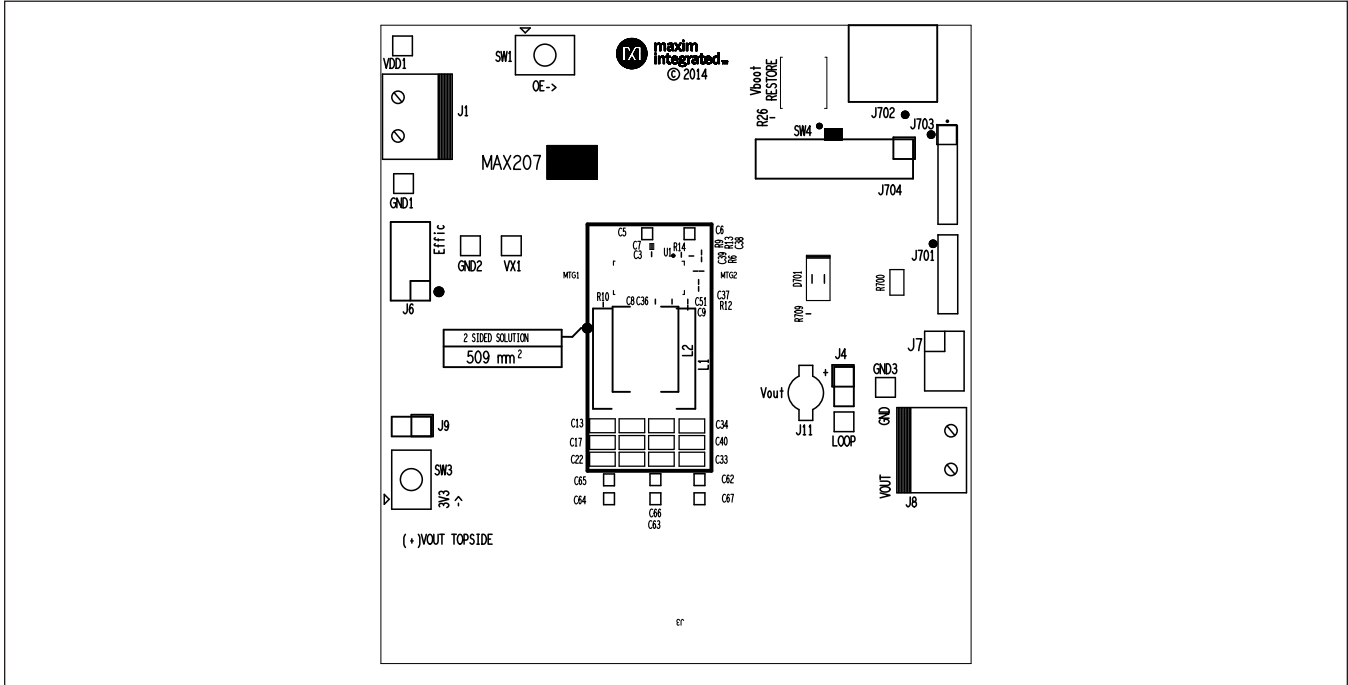
Top Silkscreen
