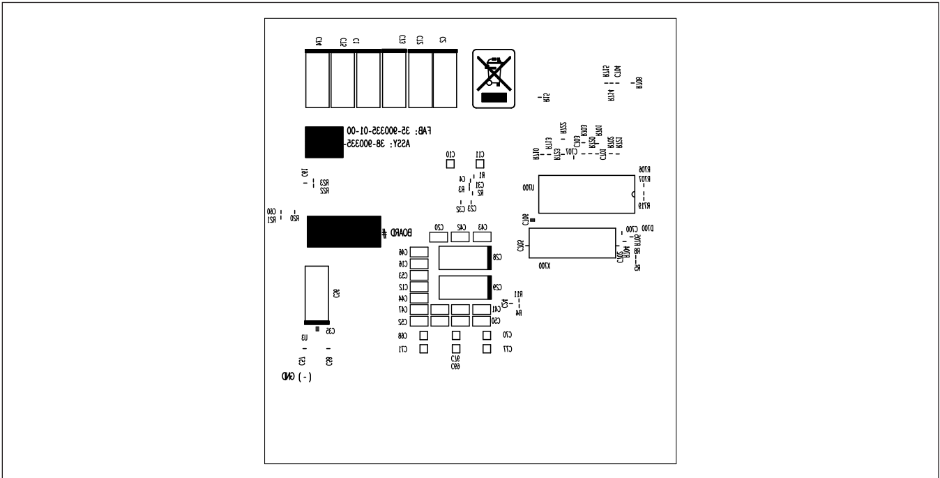
Bottom Silkscreen
