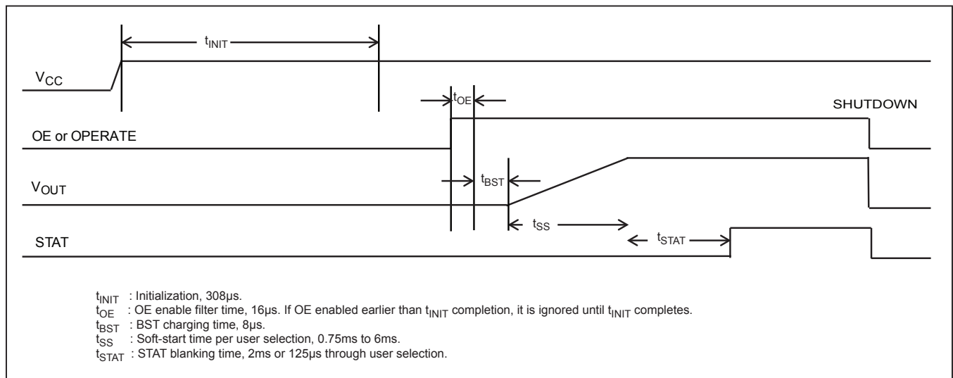
Figure 1. Startup Timing
