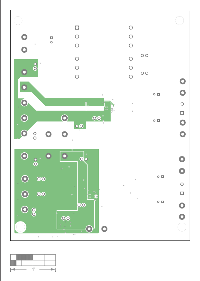
MAX22088 EV Kit—Internal Layer 3
