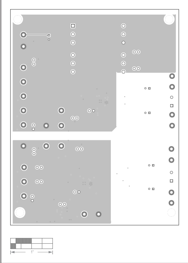
MAX22088 EV Kit—Internal Layer 2
