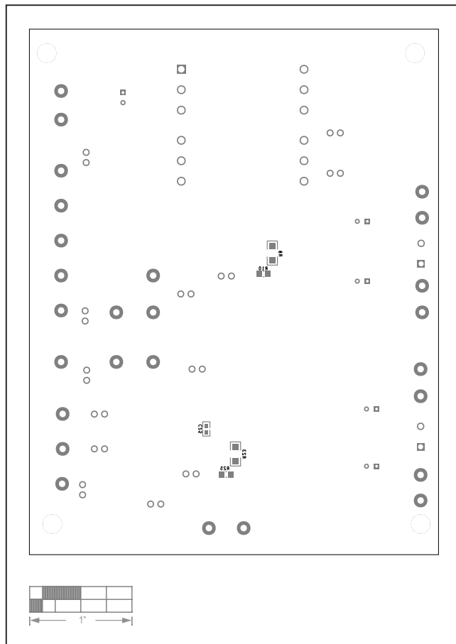
MAX22088 EV Kit—Bottom Silkscreen
