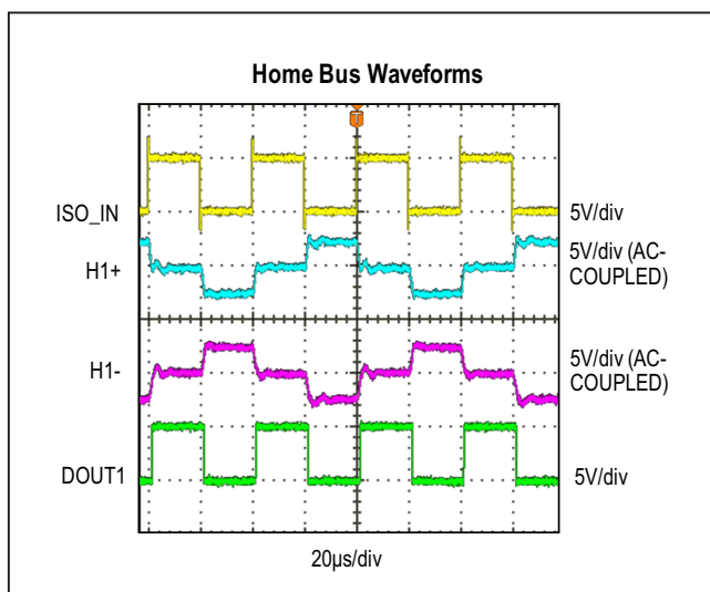
Figure 1. MAX22088 EV Kit Waveforms at 50kbps
