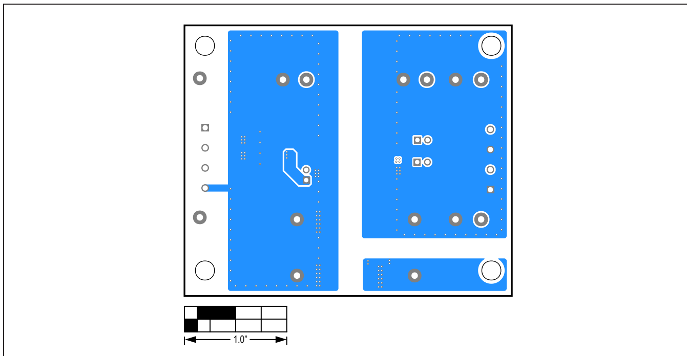
MAX22518 EV Kit PCB Layout—Bottom Layer
