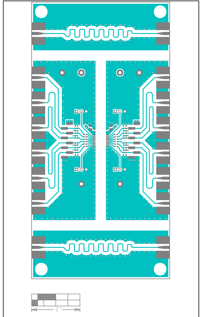
MAX22563–MAX22566 EV Kit PCB Layout—Top Layer
