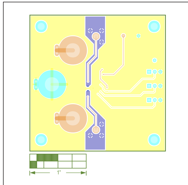
MAX25301 EV Kit—Bottom
