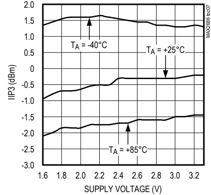
MAX2686 OUT-OF-BAND IIP3 vs. SUPPLY VOLTAGE AND TEMPERATURE (TONE 1 AT 1713MHz, -27dBm; TONE 2 AT 1851MHz, -39dBm)
