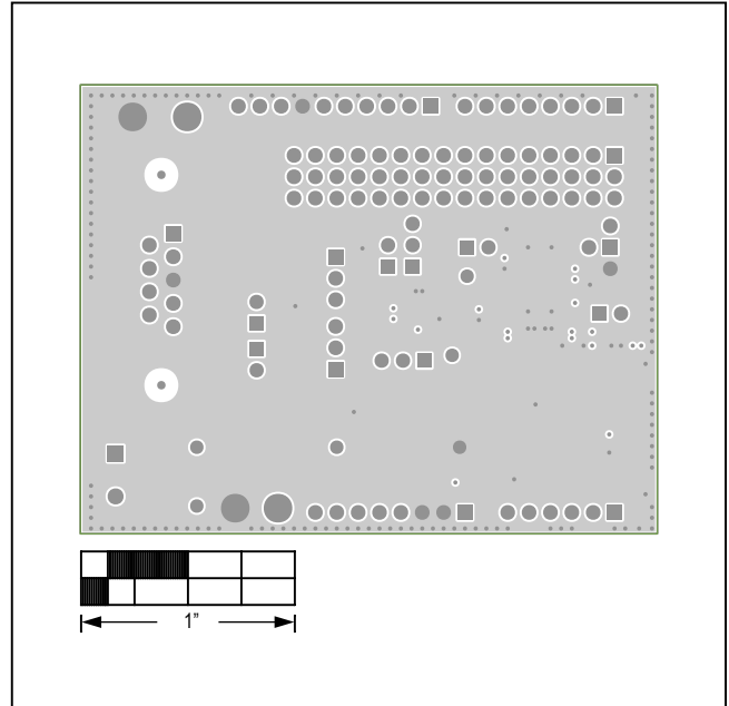
MAX33054E Shield—Internal 2
