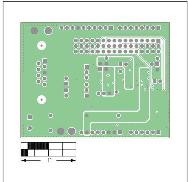
MAX33054E Shield—Internal 3
