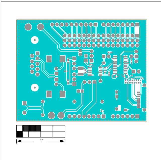
MAX33054E Shield—Top
