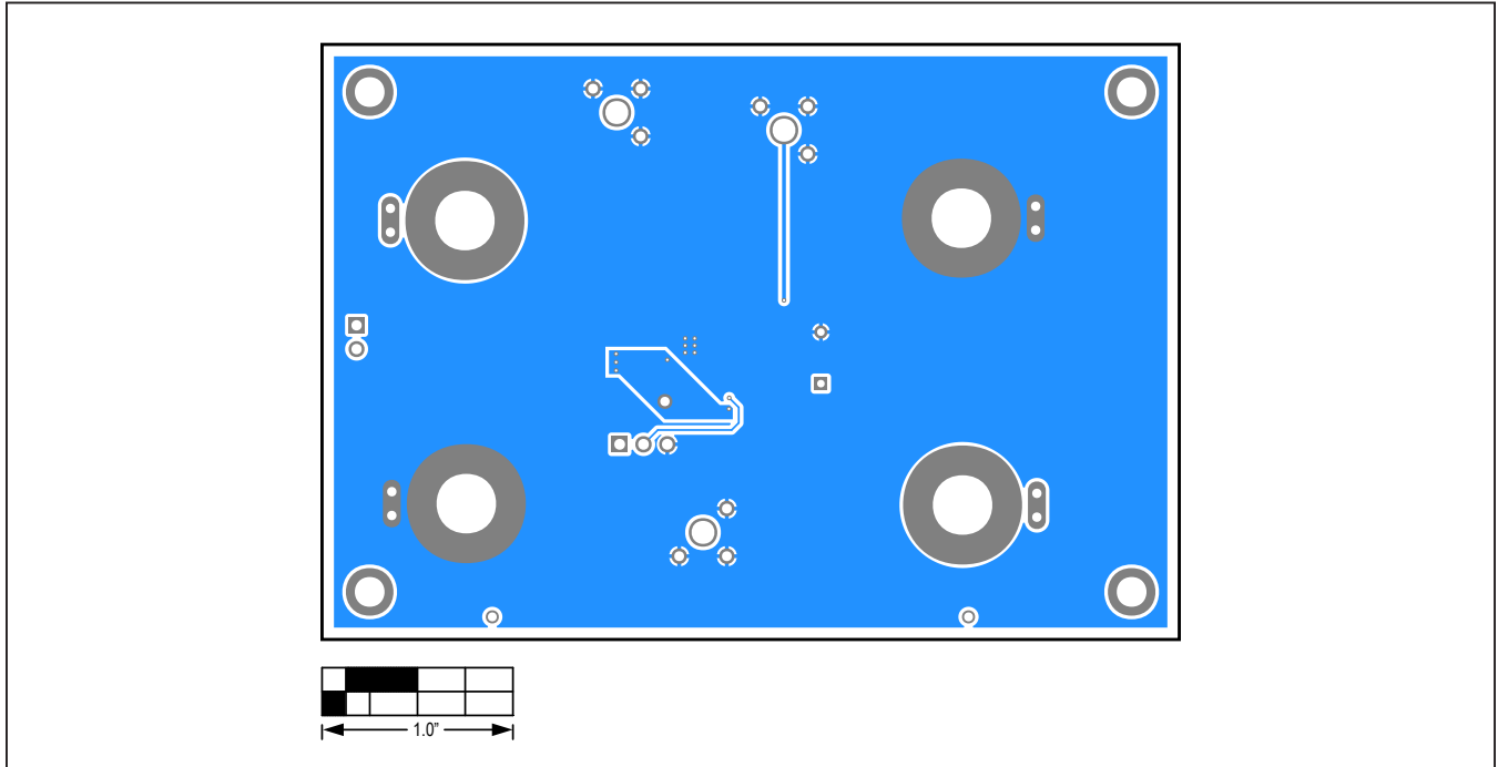
MAX38886 EV Kit PCB Layout—Bottom View
