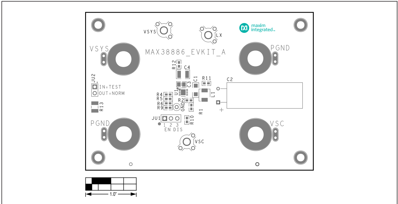
MAX38886 EV Kit Component Placement Guide—Top Silkscreen
