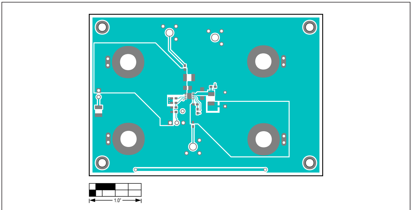
MAX38886 EV Kit PCB Layout—Top Assembly
