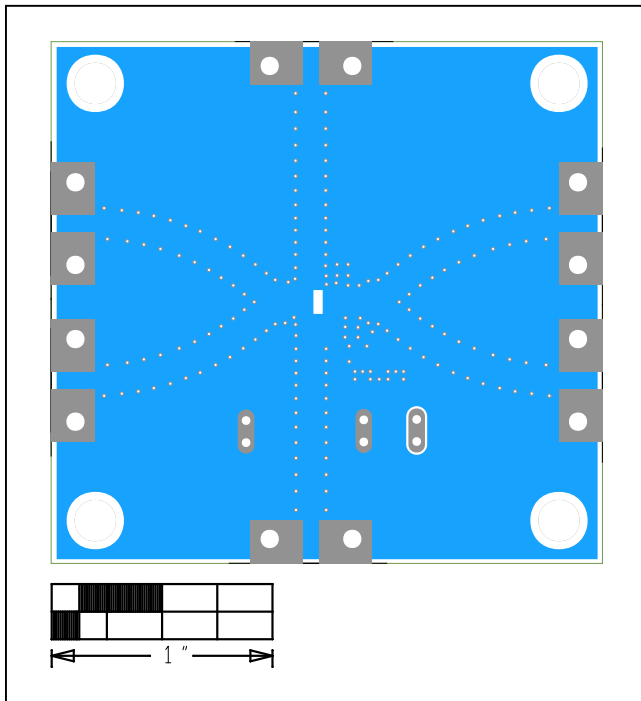
MAX40026 EV—Bottom
