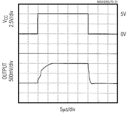
POWER-UP/POWER-DOWN RESPONSE
