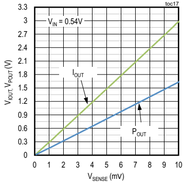
V IOUT , V POUT vs. V ISENSE ( 100\mu A , 10mV RANGES)
