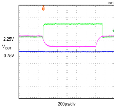
V SENSE STEP RESPONSE ( V_{SENSE} = 2.5mV TO 7.5mV , V_{IN} = 0.54V )
