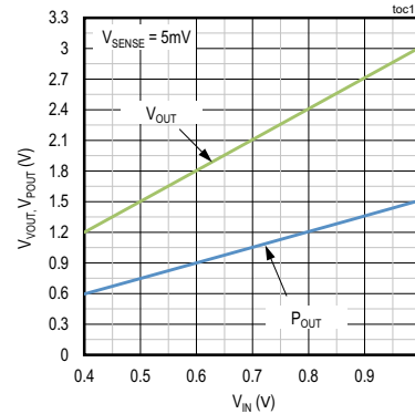
V IOUT , V POUT vs. V IN ( 100\mu A , 10mV RANGES)
