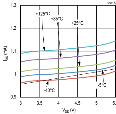
I DD vs. V DD vs TEMP ( V_{IN} = V_{SENSE} = 0V )
