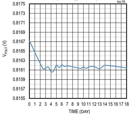
V POUT DRIFT (IC #1, T_A = +55^\circ C )
