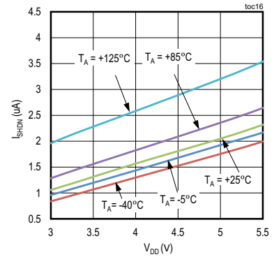
I SHDN vs. V DD vs TEMP ( V_{IN} = V_{SENSE} = 0V )
