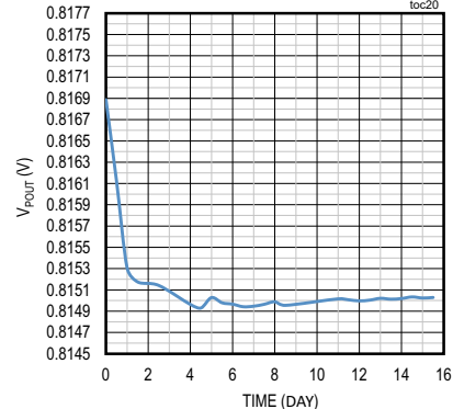
V POUT DRIFT (IC #2, T_A = +55^\circ C )
