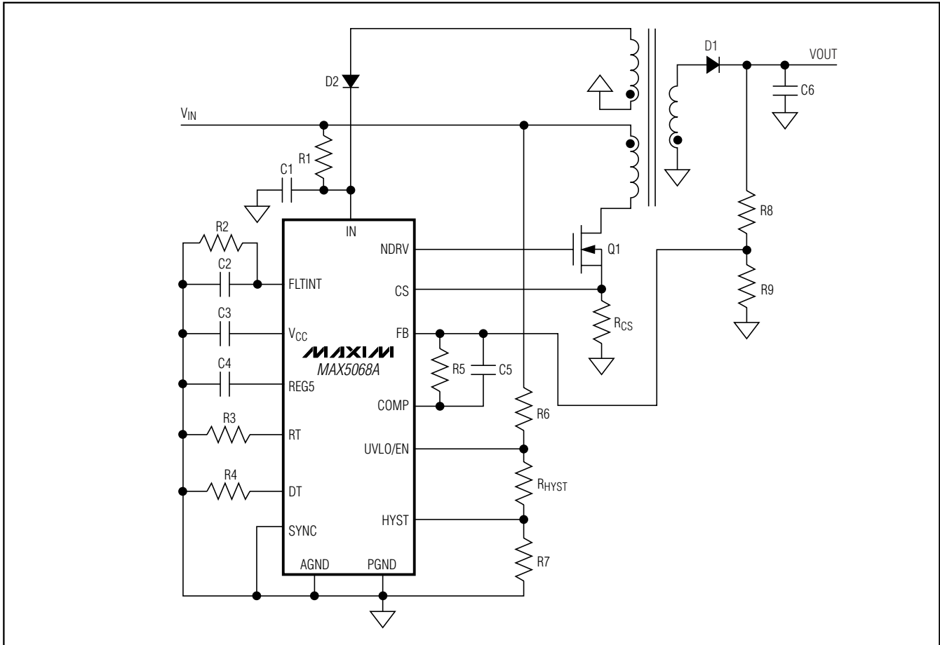
Figure 1. Nonisolated Power Supply with Programmable Input Supply Voltage
