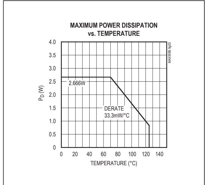
Figure 3. Calculated Maximum Power Dissipation vs. Temperature
