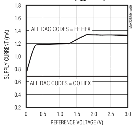
SUPPLY CURRENT vs. REFERENCE VOLTAGE (V DD = +3V)
