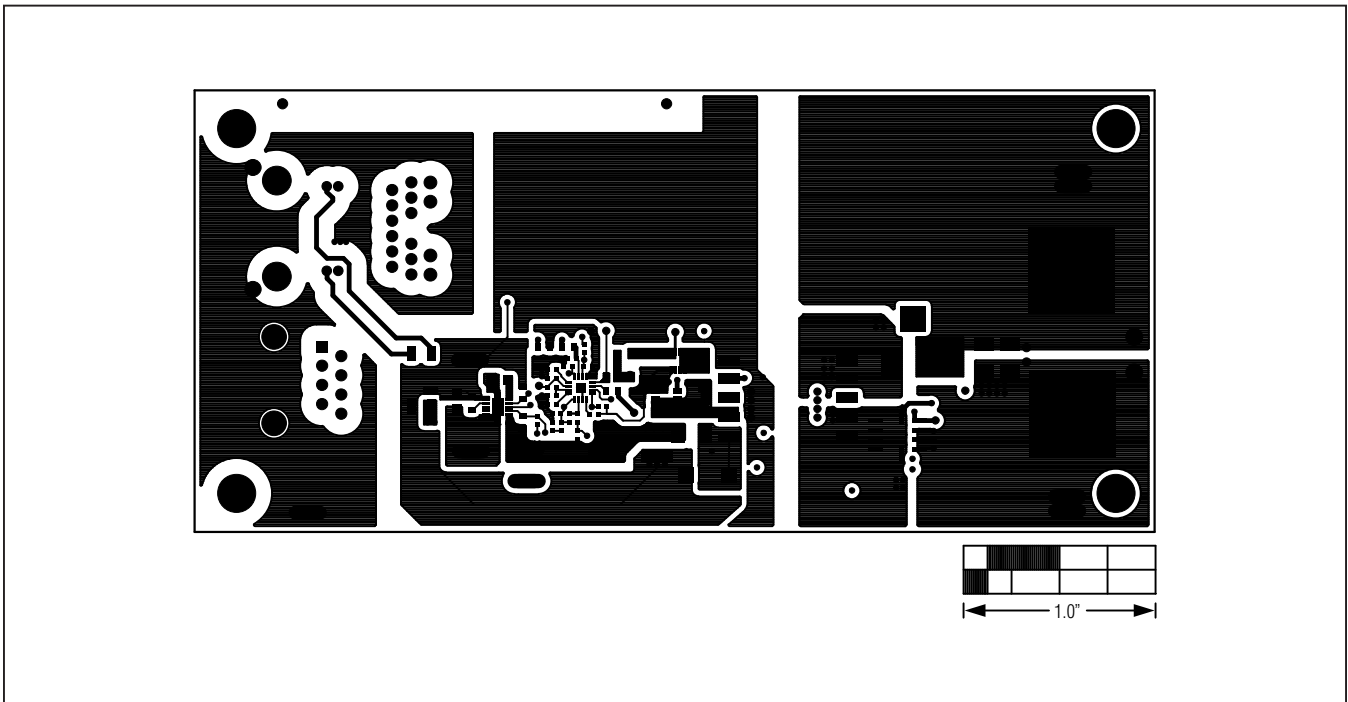
Component Side
