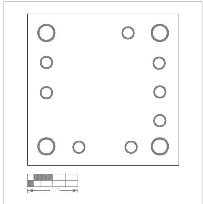
MAX6226 EV Kit Component Placement Guide—Bottom Silkscreen
