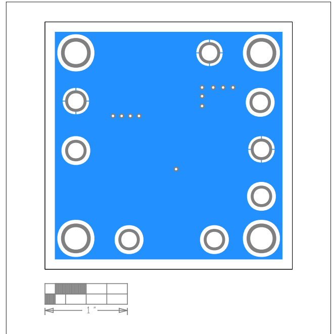
MAX6226 EV Kit PCB Layout—Bottom Layer
