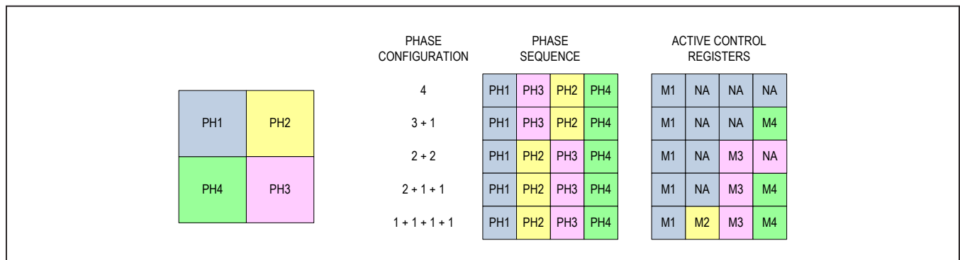
Figure 2. Buck Phase Configuration
